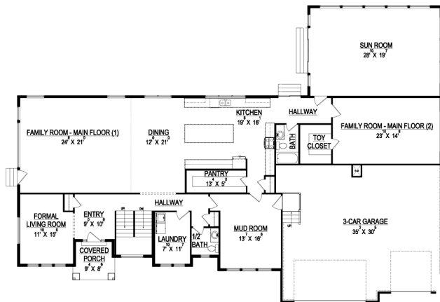
MAIN FLOOR
