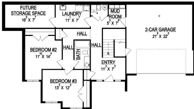
MAIN FLOOR
