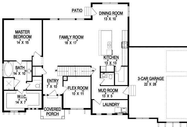
MAIN FLOOR
