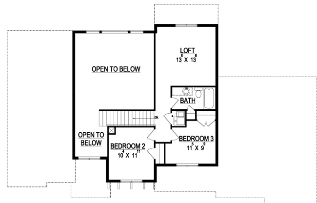
UPPER FLOOR
