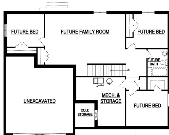
BASEMENT PLAN
