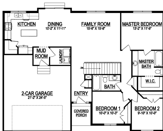
MAIN FLOOR
