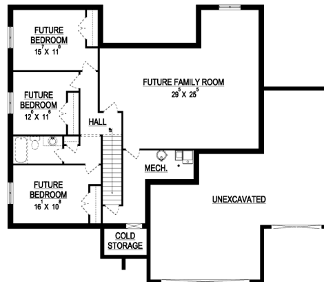
BASEMENT
