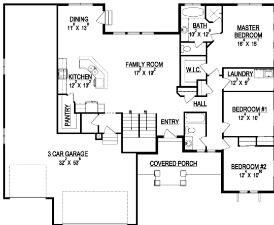
MAIN FLOOR
