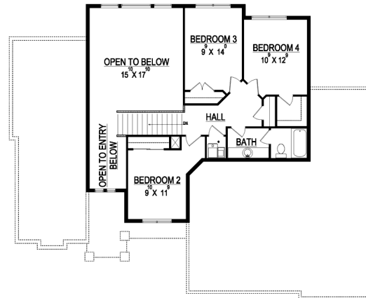
UPPER FLOOR
